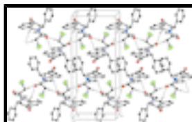
Fig. 2. The crystal packing of the title compound viewed along the a axis. H atoms not involved in hydrogen bonding have been omitted for clarity.
